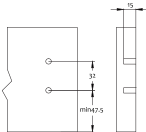
Front panel drilling dimensions
