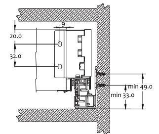
Back panel installation dimensions
