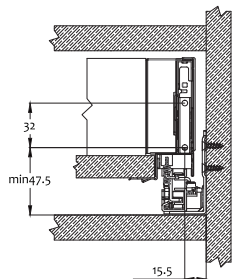
Front connector panel installation dimensions
