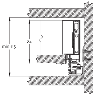
Cabinet space requirements
